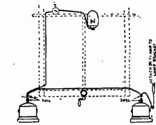
Wiring Diagram of Ford Car Furnished With Each Outfit
